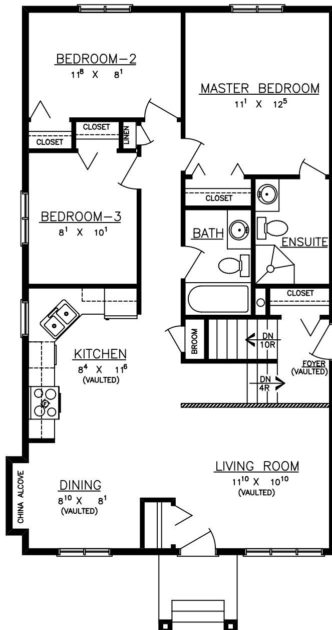
FLOOR PLAN
